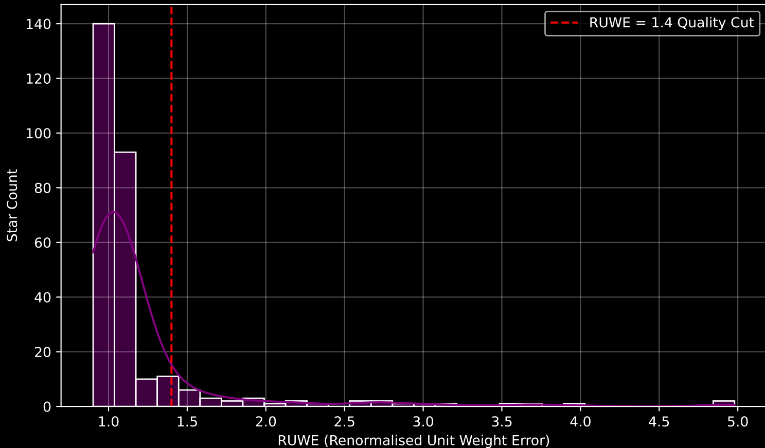
GALAH DR4 Field [236] RUWE Distribution (n= 284)
