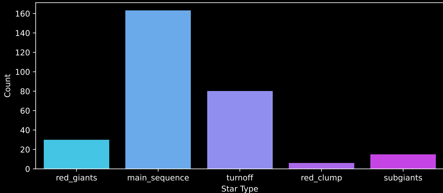
GALAH DR4 Field: [236] Count plot of Star Type
