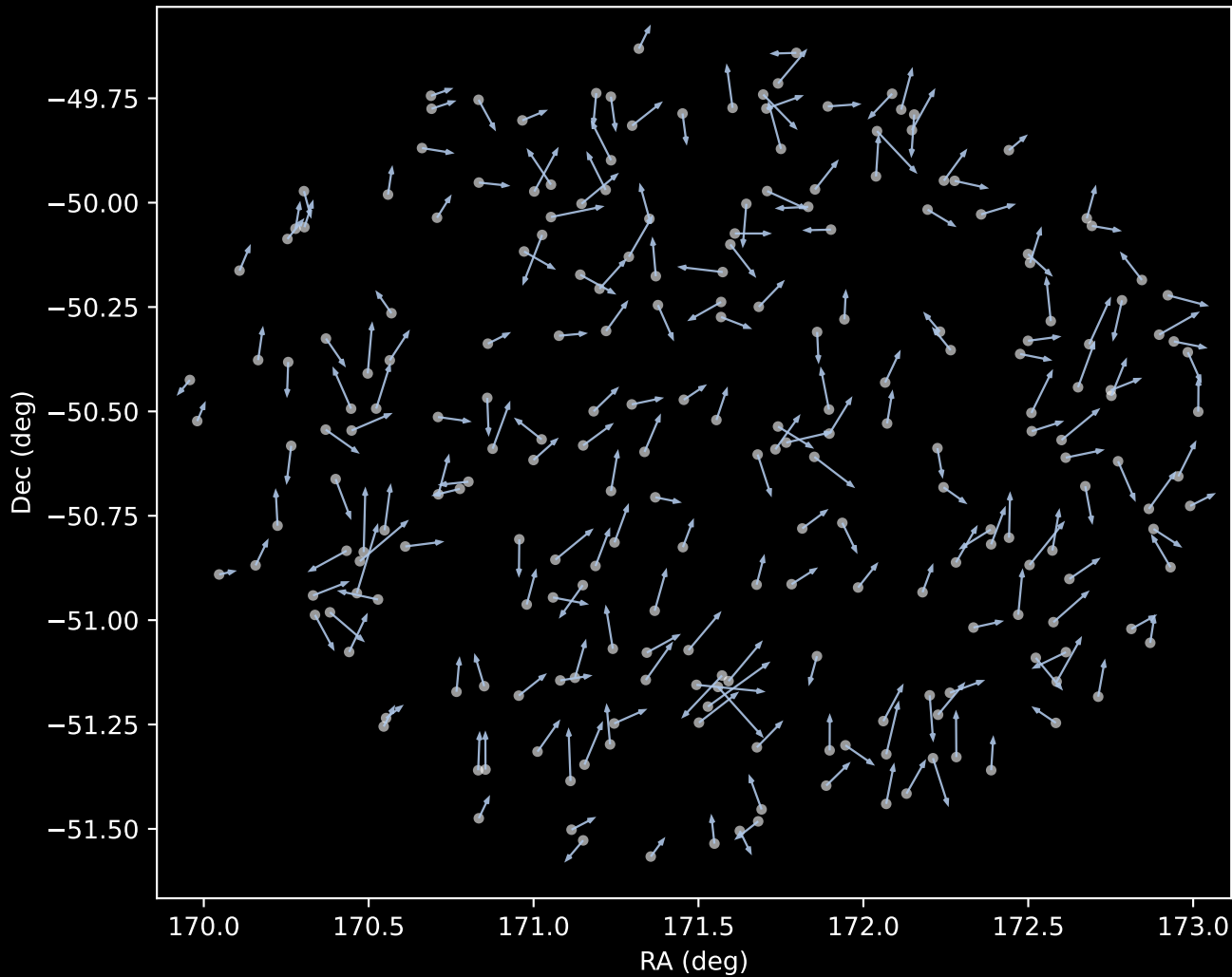
GALAH DR4 Cluster 1 Proper Motion Vectors (n=231)
